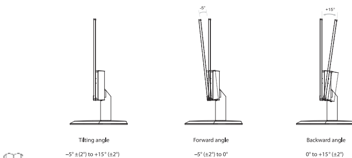
Figure 2-1 Angle adjustment
