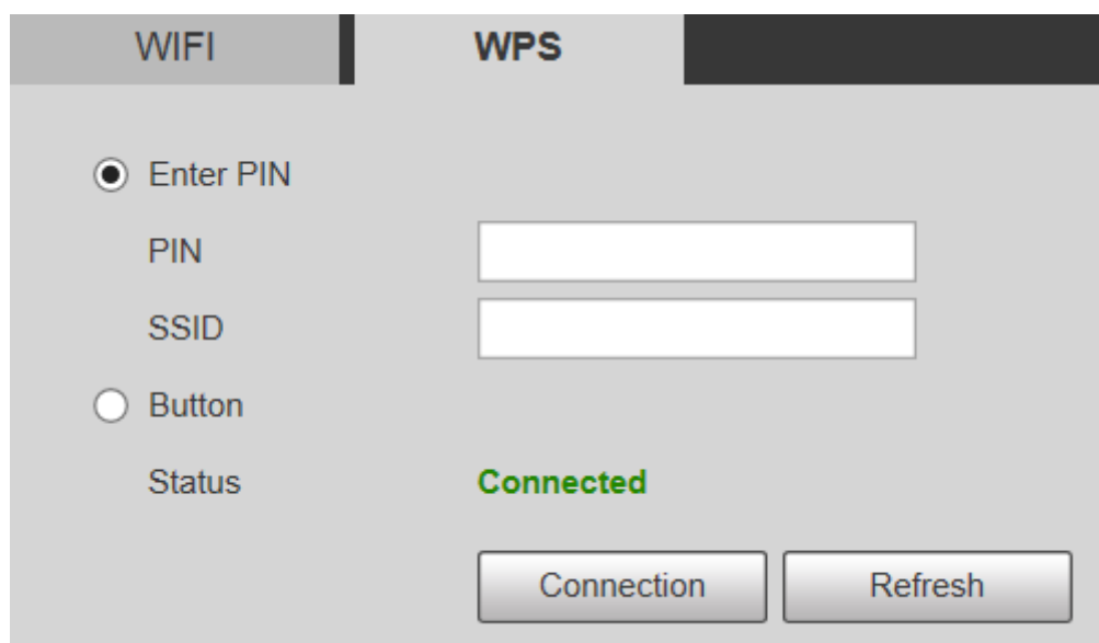
Figure 5-52 WPS setting
