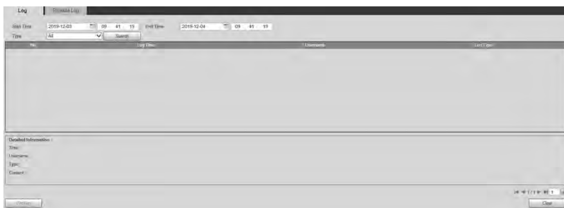
Figure 5-165 Log
