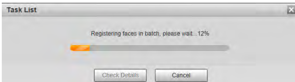
Figure 5-102 Registering
