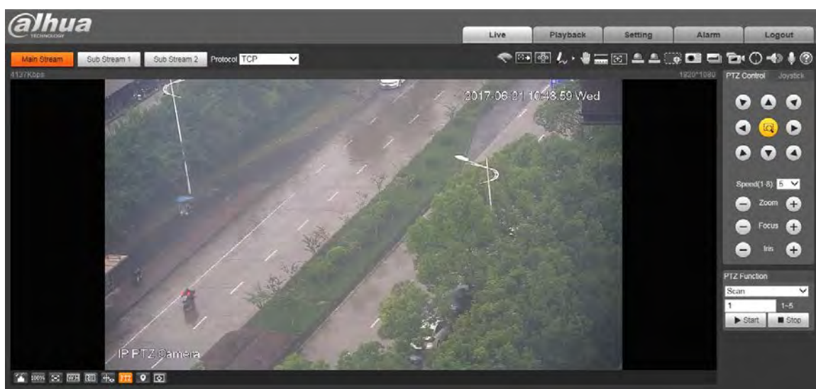
Figure 1-11 Live page
