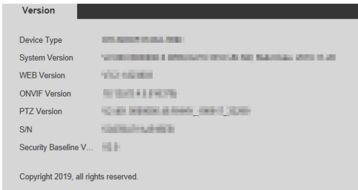
Figure 5-164 Version
