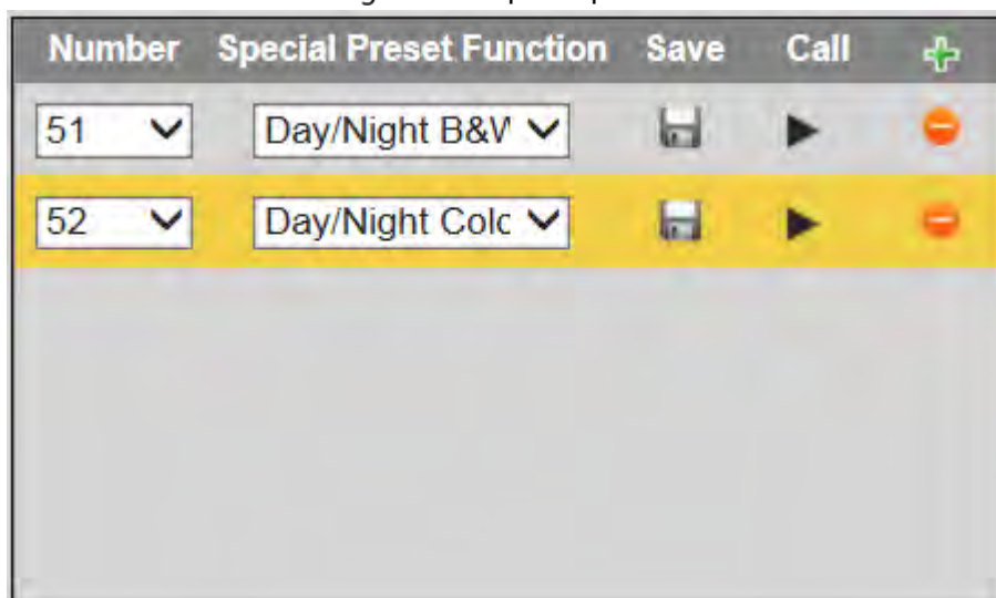
Figure 5-66 Special presets
