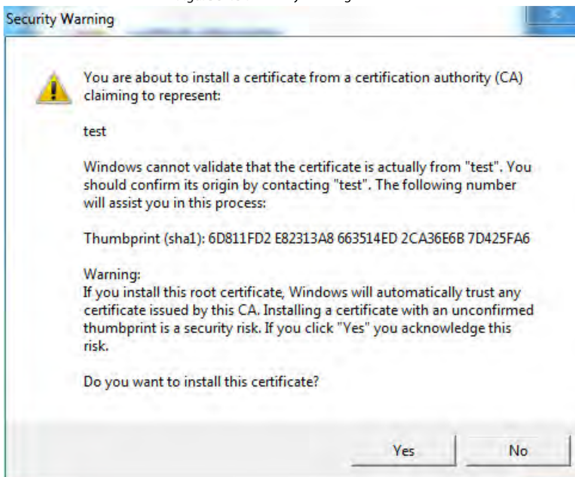
Figure 5-154 Security warning
