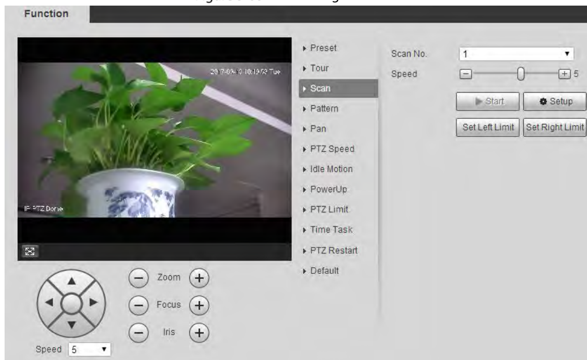
Figure 5-68 Scan settings
