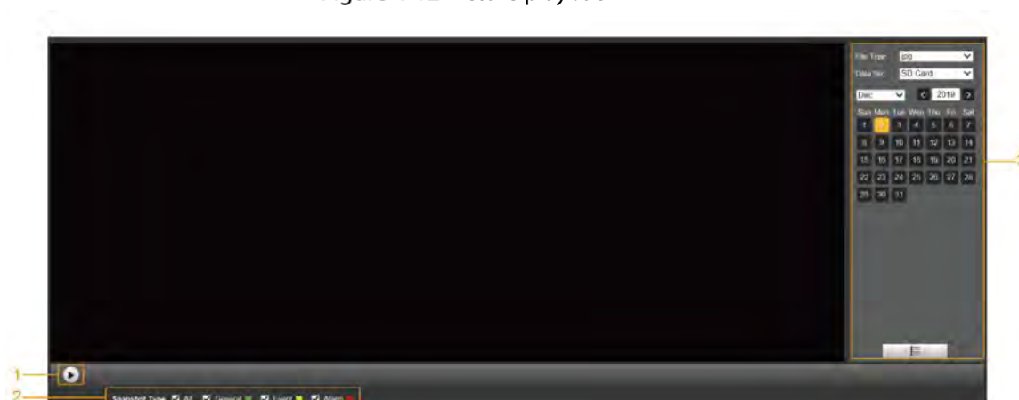
Figure 4-12 Picture playback
