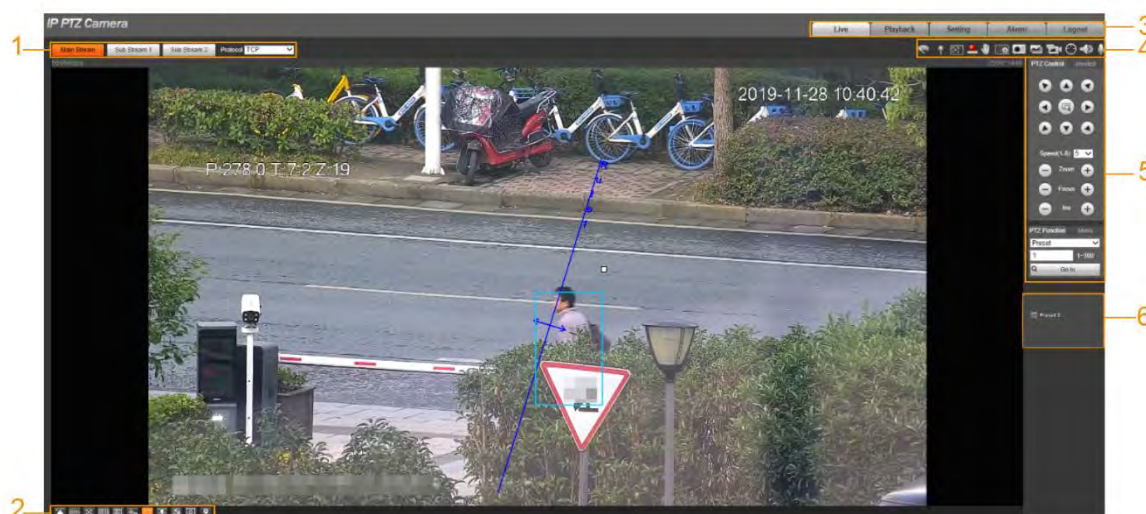
Figure 2-1 Live page
